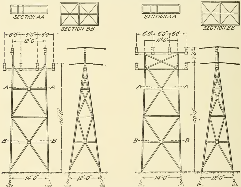
Fig. 39. Plan and Elevation of Steel Tower
